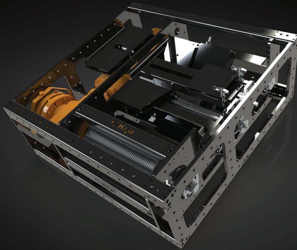
Zero Fleet Deck Winch
